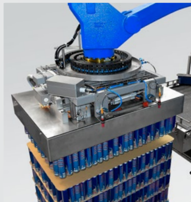
Centring & pick-up of the products
